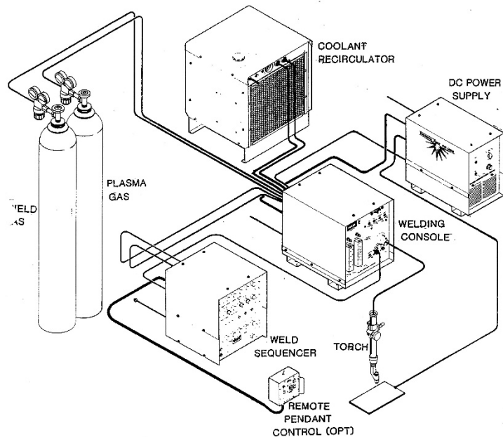
Figure 1-A Plasma Welding System
